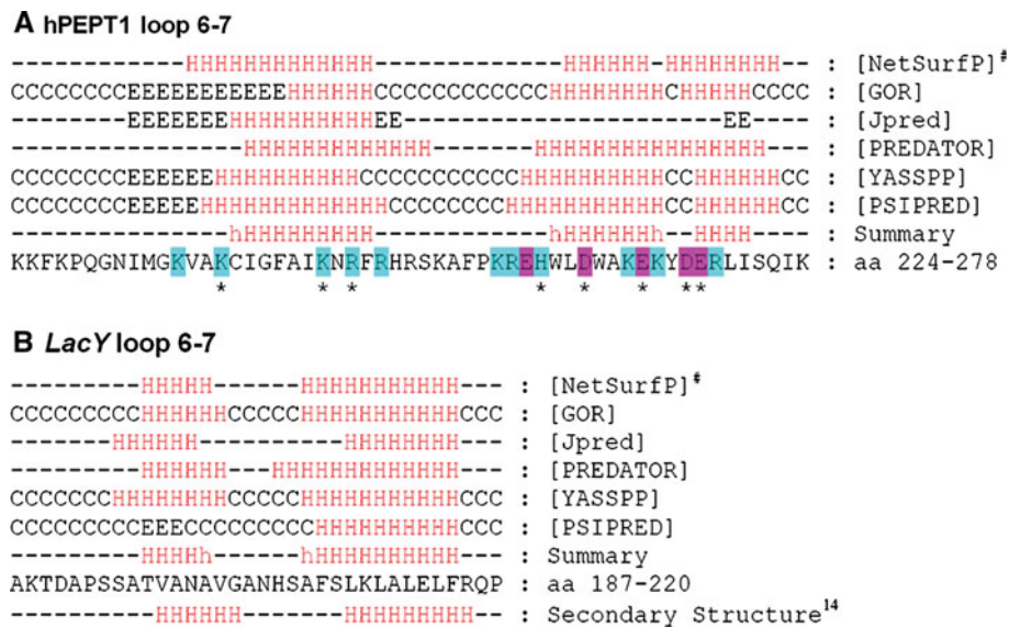
Fig. 6 Secondary structure predictions for loop 6–7 in hPEPT1 and LacY. Predictions were made using the online servers of six programs: NetSurfP (Petersen et al. 2009), GOR (Sen et al. 2005), Jpred (Cole et al. 2008), PREDATOR (Frishman and Argos 1996), YASSPP (Karypis 2006) and PSIPRED (Bryson et al. 2005). The summary was generated based on the results of these programs: H (helix) indicates at least five of the programs predicted a helix at a given position, and
