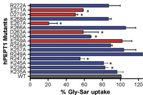
Fig. 2 Percentage of Gly-Sar uptake activities by transporters with alanine mutations of residues in loop 6–7 of hPEPT1 relative to WT-hPEPT1 ( n = 4–7 experiments per mutation). [ ^3\text{H} ]Gly-Sar uptake (0.5 \mu\text{Ci/ml} , 10 min at 37^\circ\text{C} ) was measured 72 h posttransfection in HEK293 cells. Background uptake of mock-transfected HEK293 cells was subtracted. *P < 0.05 vs. WT-hPEPT1 uptake
