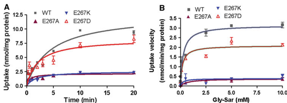
Fig. 5 a Time courses of Gly-Sar uptake by WT-hPEPT1 (gray) and E267D (red), E267A (purple) and E267K (blue) mutants ( n \geq 3 for each point). b Concentration dependence of Gly-Sar uptake by WT-hPEPT1
