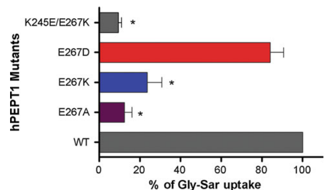
Fig. 3 Percentage of Gly-Sar uptake by transporters with E267 mutations relative to WT-hPEPT1. *P < 0.05 vs. WT-hPEPT1
