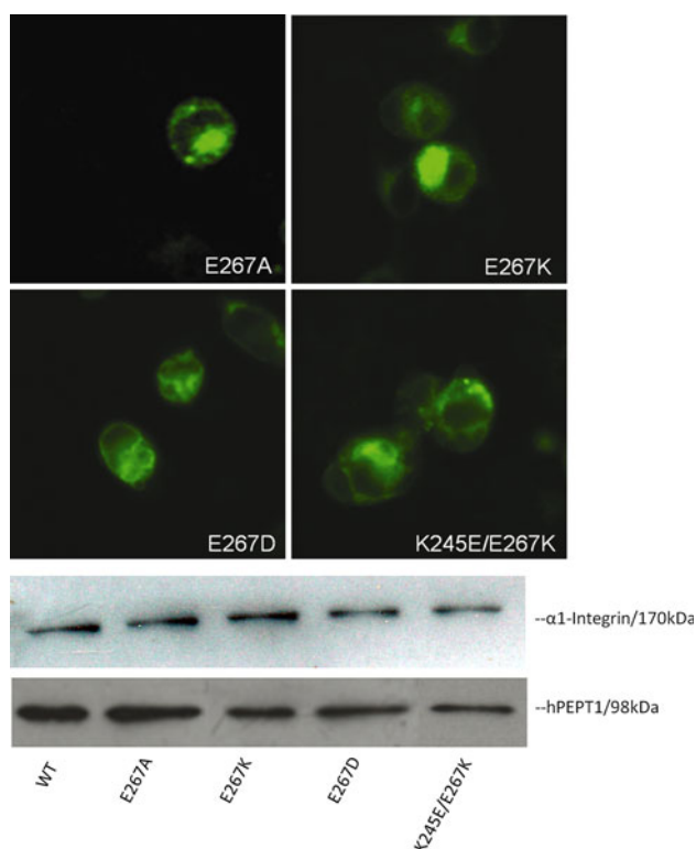
Fig. 4 Membrane expression of mutants at E267 of hPEPT1 in transiently transfected HEK293 cells after 72 h posttransfection. Membrane localization was visualized with affinity-purified rabbit anti-hPEPT1 primary antibody (1:200) and FITC-conjugated secondary antibody (1:200). HEK293 cells with transfected proteins were biotinylated with sulfo-NHS-LC biotin for 30 min at room temperature. Immunoprecipitation was carried out, followed by Western blot analysis using affinity-purified rabbit anti-hPEPT1 primary antibody (1:500), with visualization using goat anti-rabbit HRP-conjugated secondary antibody (1:10,000) and chemiluminescence. \alpha_1 -integrin (1:10,000) was used as the internal control
